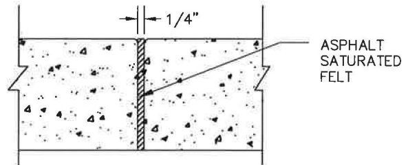
TYPICAL EXPANSION JOINT
