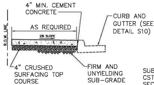
TYPICAL SECTION
